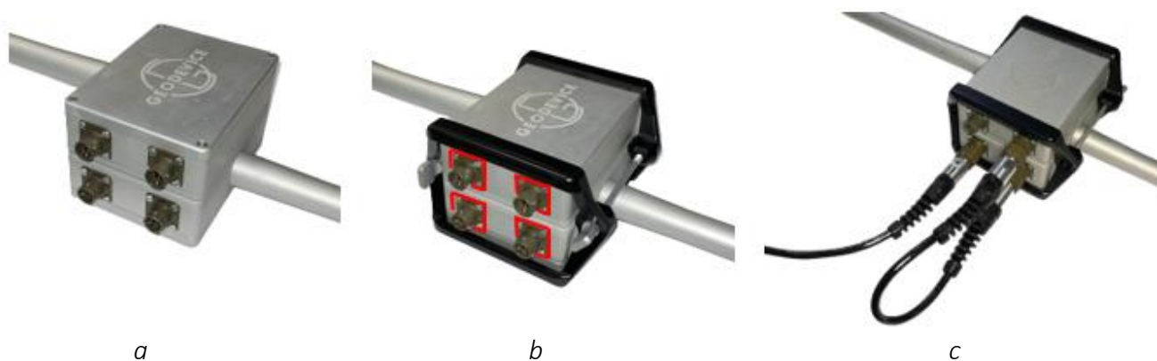
Figure 30 Assembling two OVHmag sensors into a magnetometer- gradiometer
