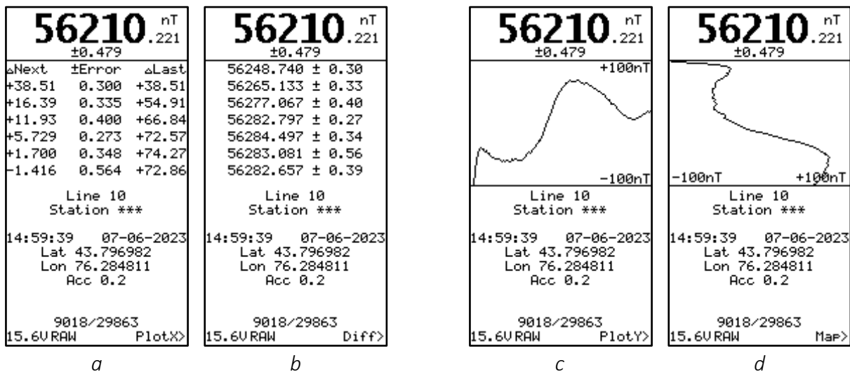
Figure 66 Found data window with different modes of displaying
