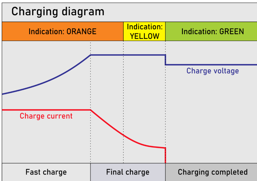
Figure 130 Charge diagram
