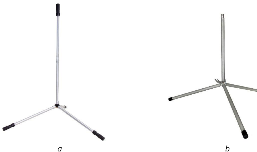
Figure 80 Assembled non-magnetic tripod a – before year 2023 model, b – after year 2022 model
