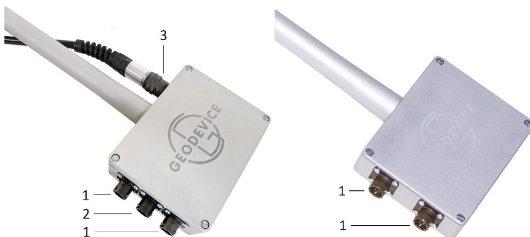
Figure 8 OVHmag electronics unit with a sensor on cable (left) and on rod (right)
