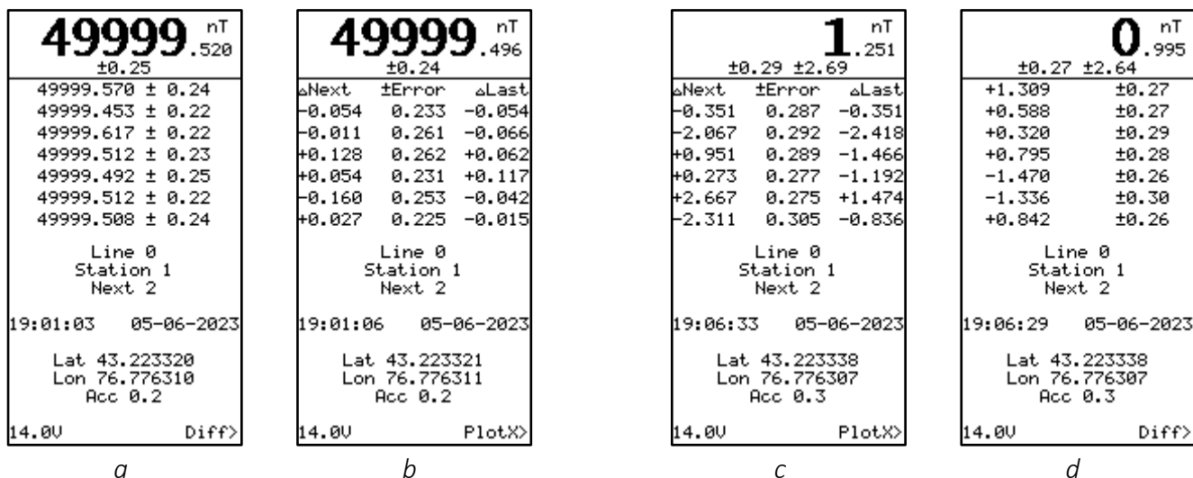
Figure 53 Measurement window in the Mobile survey mode a,b – with one sensor; c,d – with two sensors
