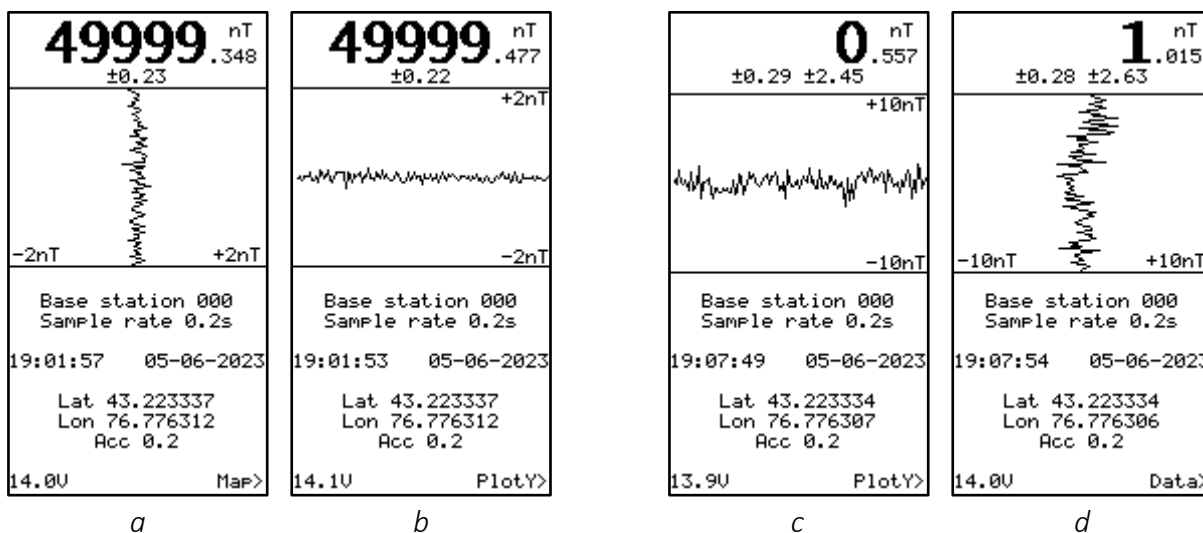
Figure 60 Window with a graph of measurements in the Base station mode a, b – horizontal and vertical display with one sensor; c, d – horizontal and vertical display in gradiometer mode;
