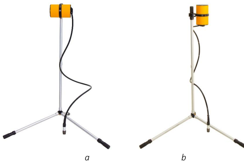
Figure 81 Assembled non-magnetic tripod a – horizontal position of the sensor; b – vertical position of the sensor
