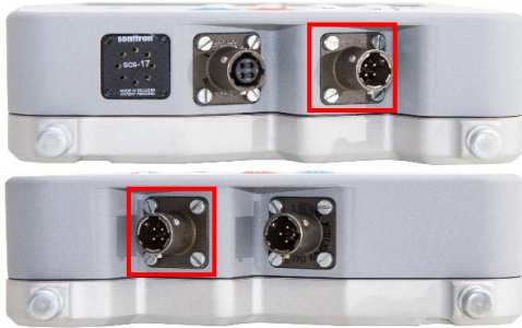
Figure 23 CAN FD + 12V connectors for connecting sensor cable on the console
