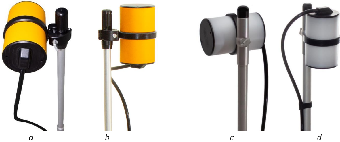
Figure 82 Overhauser sensor fixed on the non-magnetic tripod a – before year 2023 model, b – after year 2022 model
